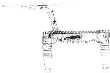
LT8700 BLACK PAINTED LIFT MECHANISM
